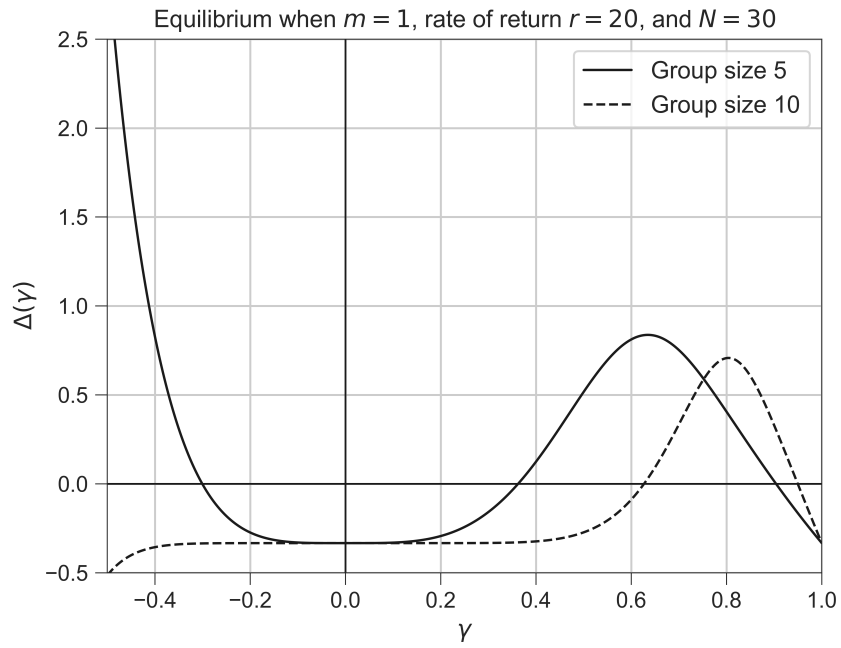
Figure 2: Mixed Strategy Equilibrium-Comparing group sizes
