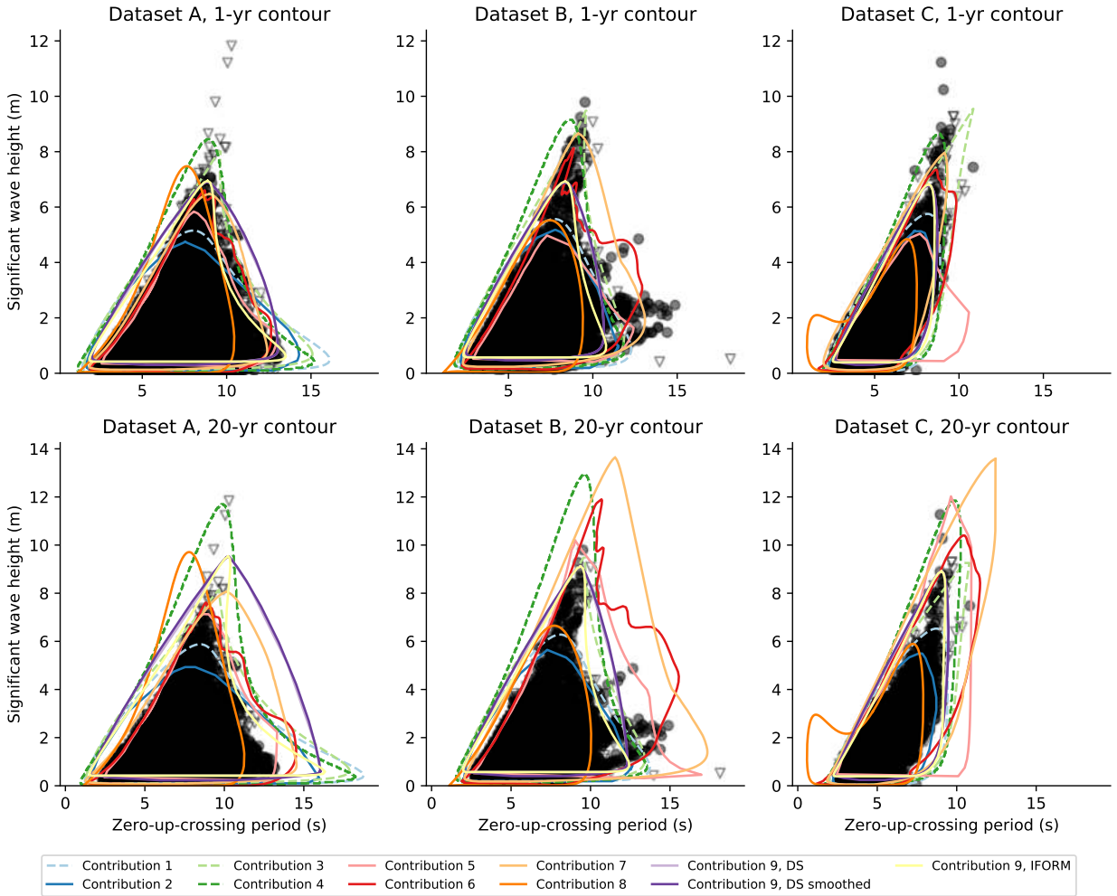
Figure 7: Exercise 1, datasets A , B , C : contour overlays. — = marginal exceedance contours, -- = total exceedance contours, ○ = provided data (10 years), ▽ = retained data (10 years).
