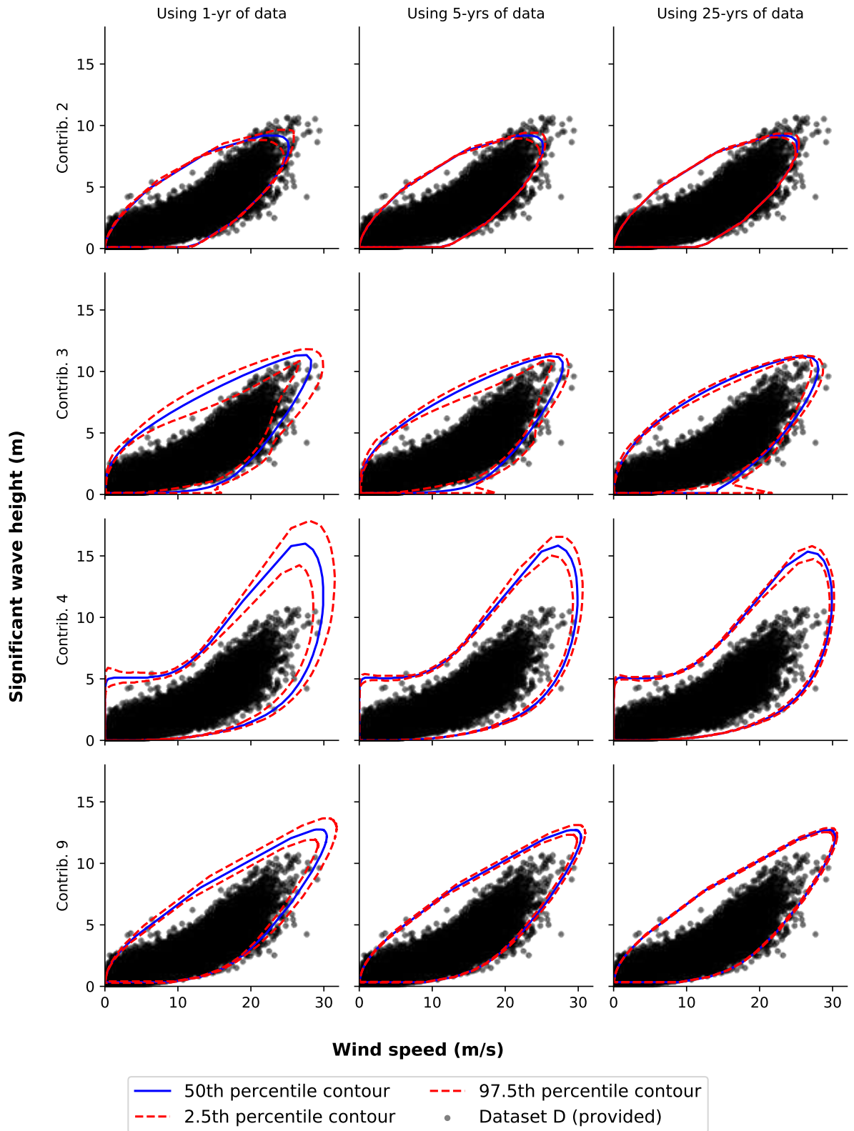
Figure 12: Exercise 2: Sampling uncertainty of the 50-yr contours. Each row of plots relates to a specific contribution (2, 3, 4, and 9); each column relates to the amount of data used to produce the 50-yr contours (1, 5, and 25 years).
