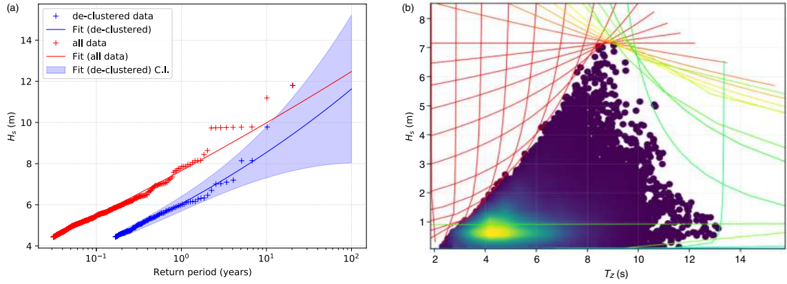
Figure 5: D-IFORM (contribution 5) illustration, Dataset A. (a) Effect of de-clustering. (b) Contour construction from tangents (transformed back in physical plane).
