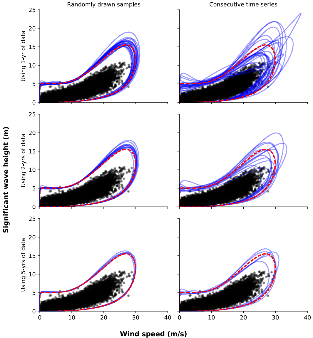
Figure 16: Effect of the metocean data's autocorrelation in Exercise 2. As an example contour method 4 is used. Left: 25 contours that are constructed by randomly sampling 1, 2 and 5 years of observations from dataset D as prescribed in Exercise 2. Right: 25 contours constructed from 1-yr, 2-yr and 5-yr consecutive sequences of dataset D . Continuous lines = contours based on 1-yr, 2-yr and 5-yr datasets, dashed line = contour based on the full consecutive 25-yr time series.
