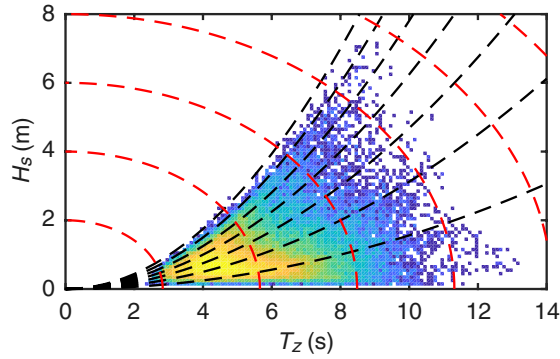
Figure 6: Joint occurrence of H_s and T_z for dataset A. Black dashed lines: constant significant steepness. Red dashed lines: constant distance d = \sqrt{H_s^2 + T_z^2/2} .
