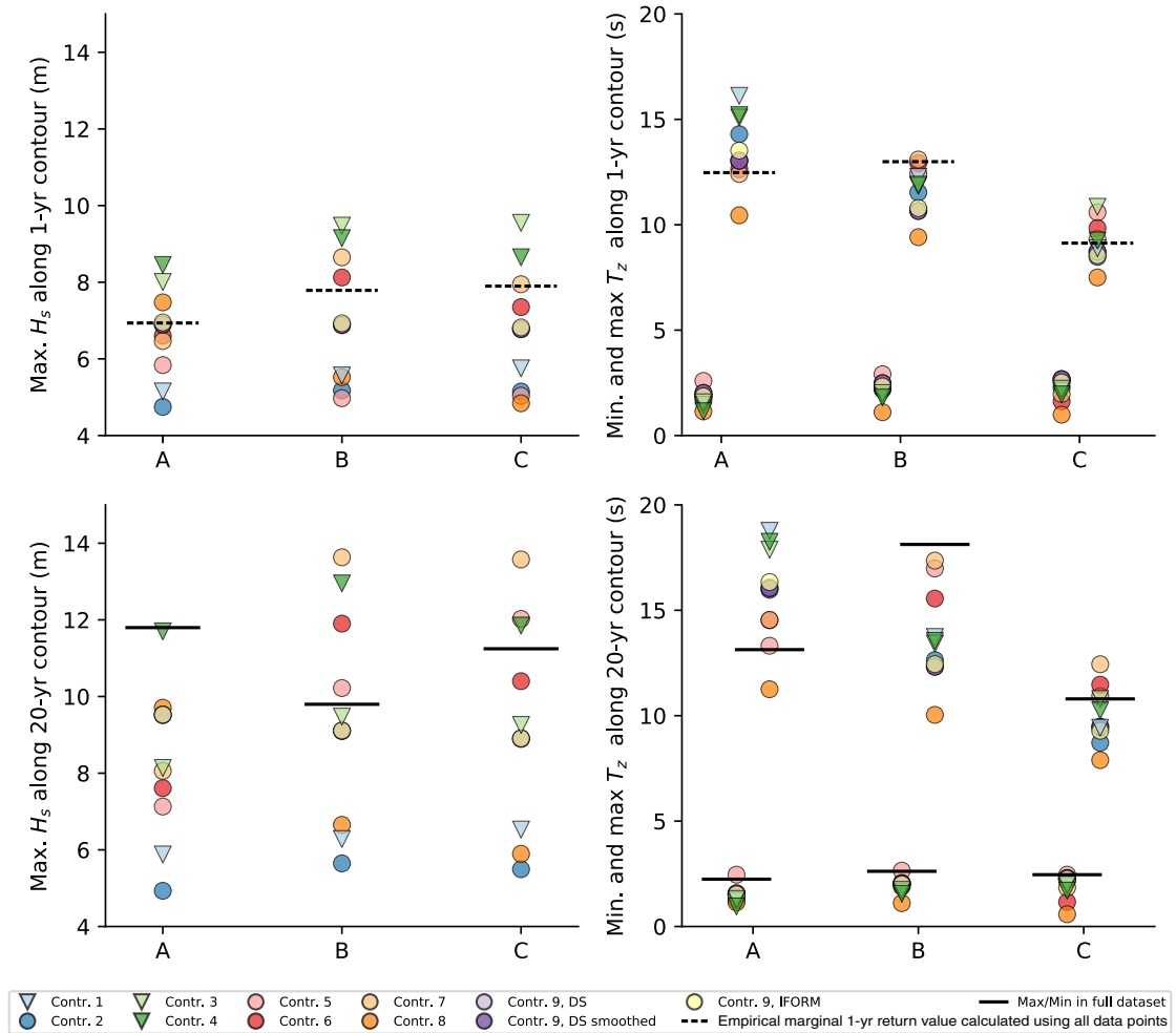
Figure 8: Exercise 1, maximum values along the contour for datasets A , B , C . For zero-up-crossing period, T_z , the minima are shown too (there is no horizontal line for the 1-yr minimum in the top right panel because the dashed lines in this figure represent the marginal 1-yr return value). \circ = marginal exceedance contours (IFORM, direct sampling, direct IFORM), \nabla = total exceedance contours (ISORM, inverse directional simulation, highest density).
