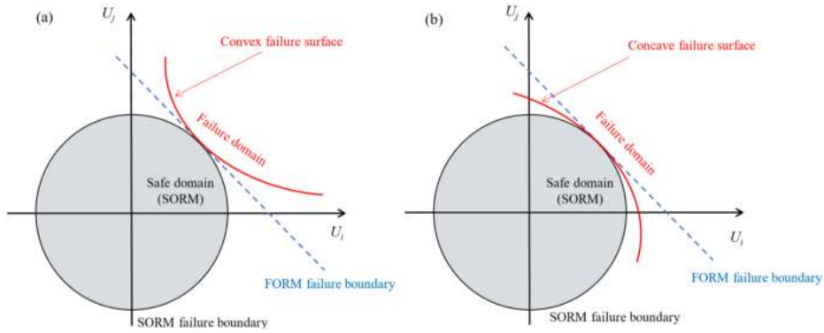
Figure 4: Illustration of failure probability approximated by the FORM and proposed specific SORM in the normalized U -space.
