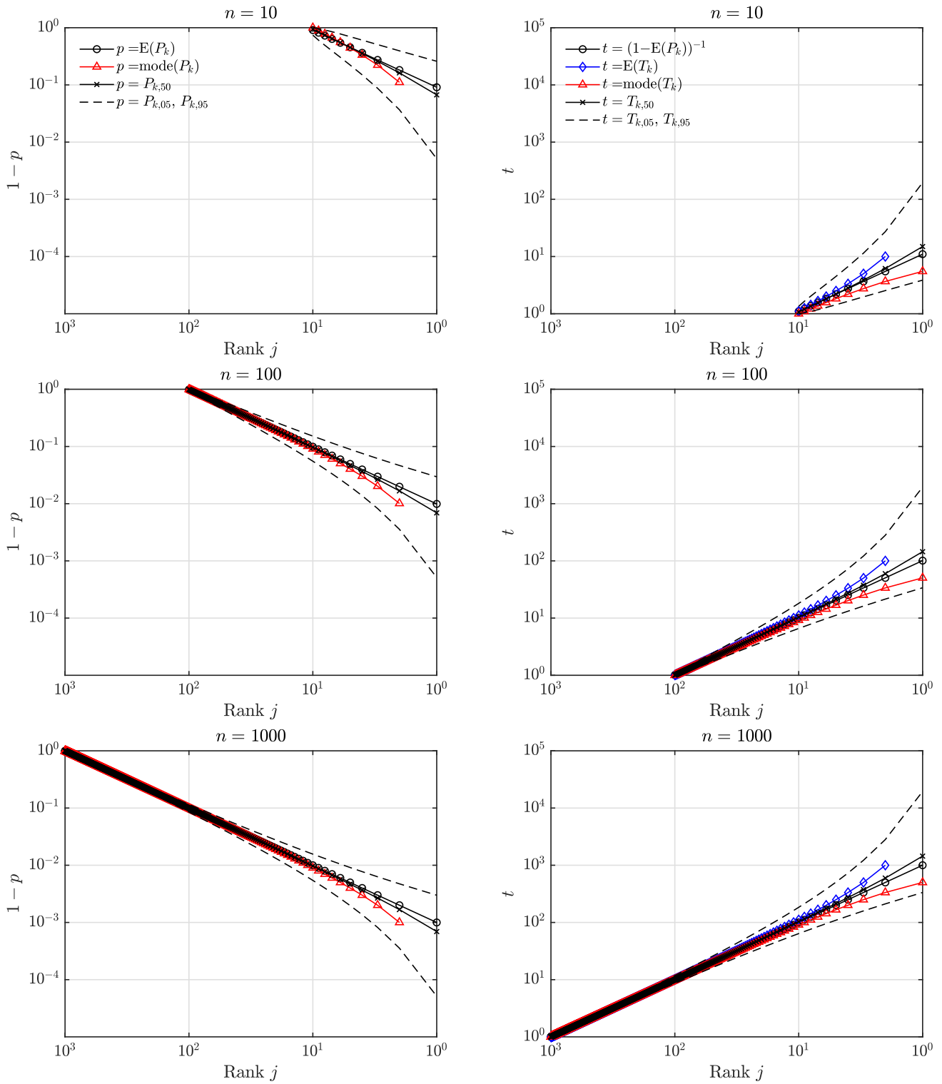
Figure 2: Values of various statistics of P_k and T_k against rank j = n - k + 1 (i.e. j = 1 is the largest observation) for various sample sizes, n .
