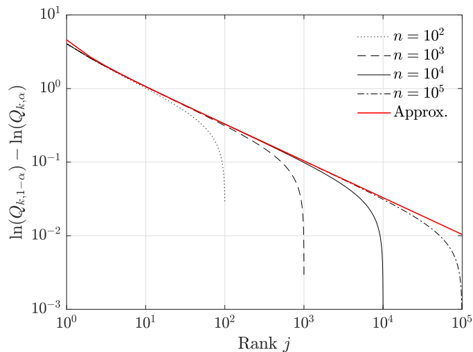
Figure 4: Width of 90% confidence interval for exceedance probabilities against rank j for various samples sizes and asymptotic approximation (22).
