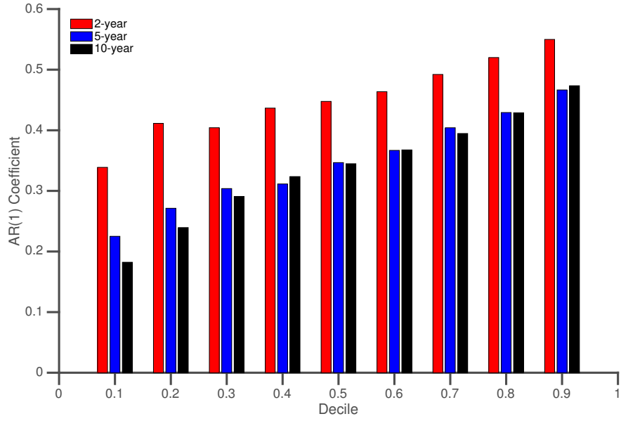
(a) \rho_i^n
