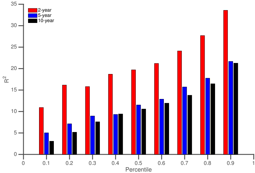
(b) R^2
