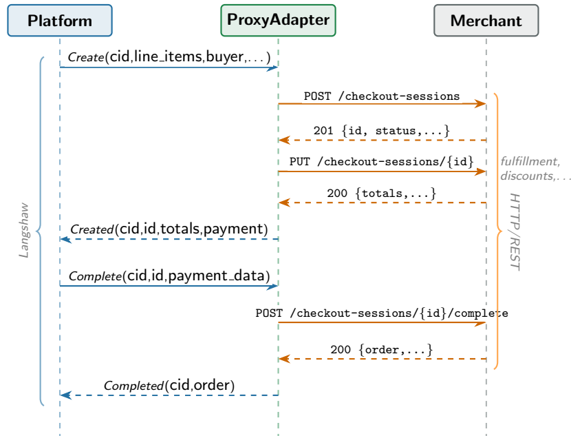
Fig. 2. Interactions for a SimpleUCP checkout via the ProxyAdapter. PLATFORM speaks Langshaw; the proxy bridges to the merchant’s HTTP API using its built-in field mapping. The proxy-internal PUT supplies fields (e.g., discounts and fulfillment) that UCP does not accept in the initial POST. Solid arrows: requests; dashed: responses.
