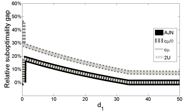
Fig. 3. Relative suboptimality gap in Scenario 3
