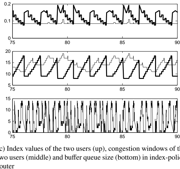
Figure 7: Scenario 3: Simulation of a bottleneck link with two users, where User1 has a TCP with \gamma_1 = 0.9 and User2 has standard TCP ( \gamma_2 = 0.5 )
