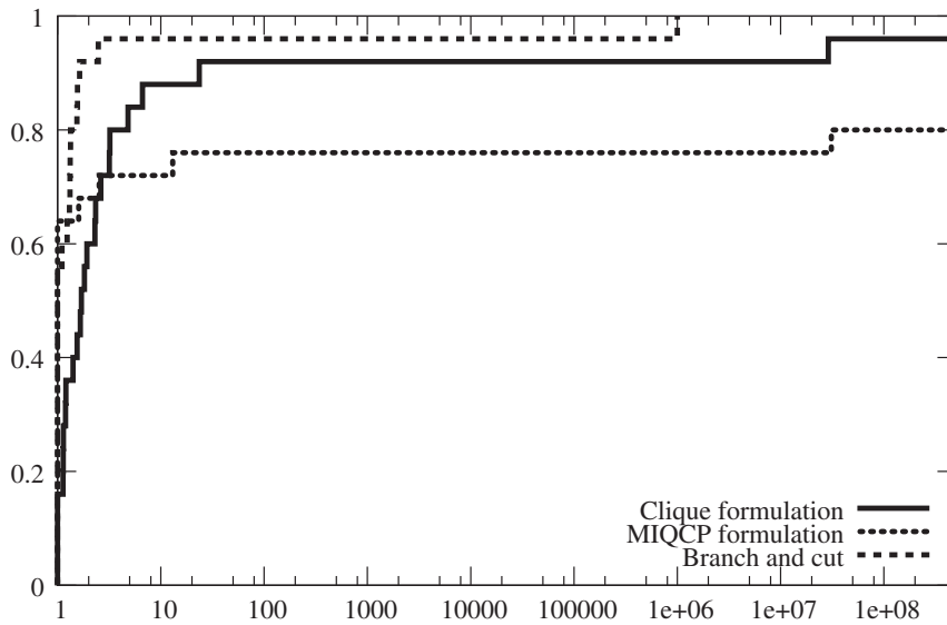
FIG. 1. Performance profile of number of subproblems.
