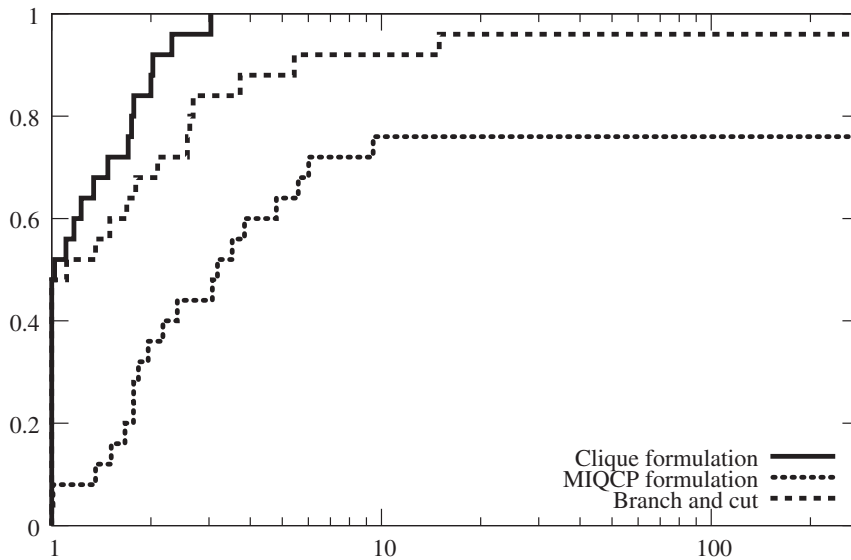
FIG. 2. Performance profile CPU time.
