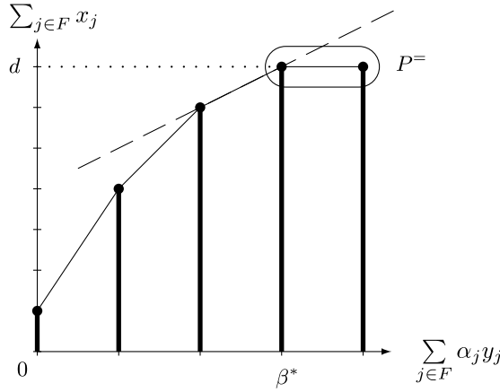
Fig. 1. Projection of feasible points onto 2-dimensional subspace.
